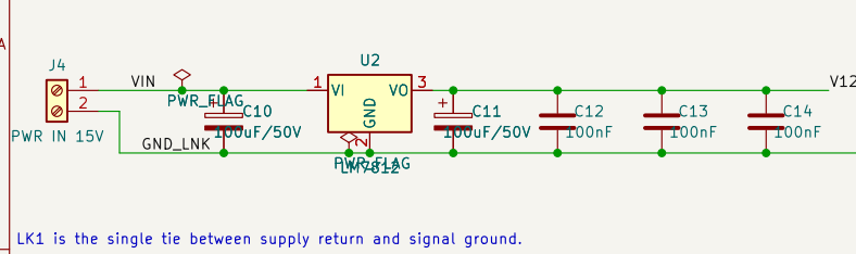
A POWER IN +15 V -> LM7812 -> +12 V
