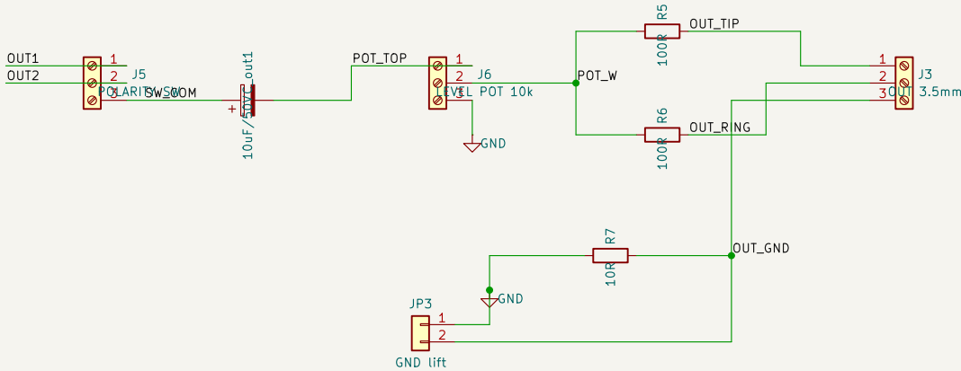
G OUTPUT polarity select -> level -> jack
