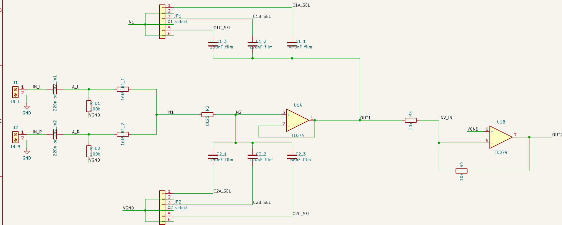
D INPUTS L + R, DC-blocked, summed
