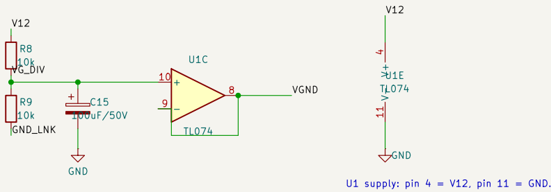
C VIRTUAL GROUND +6 V, buffered
